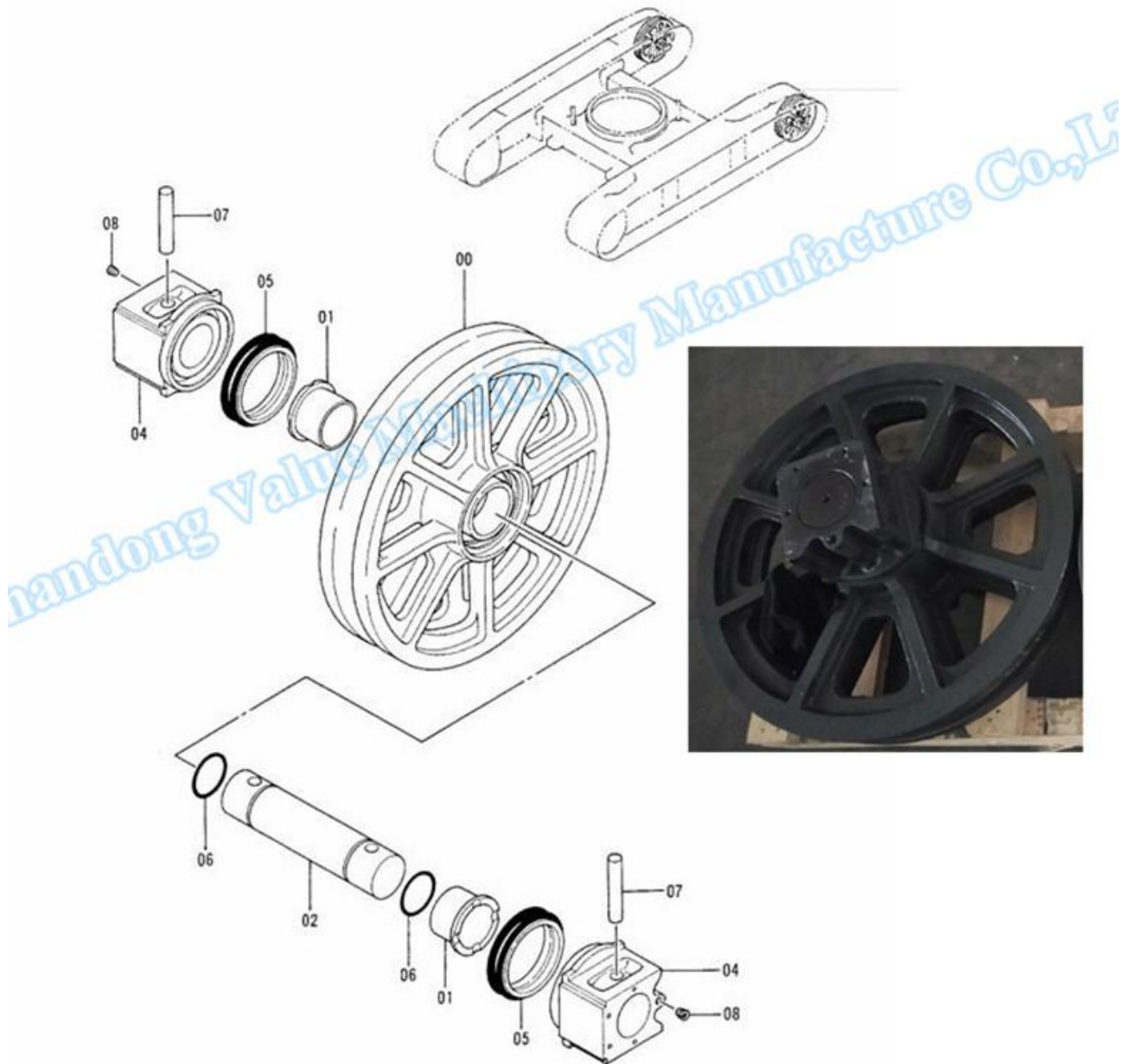
FRONT IDLER
